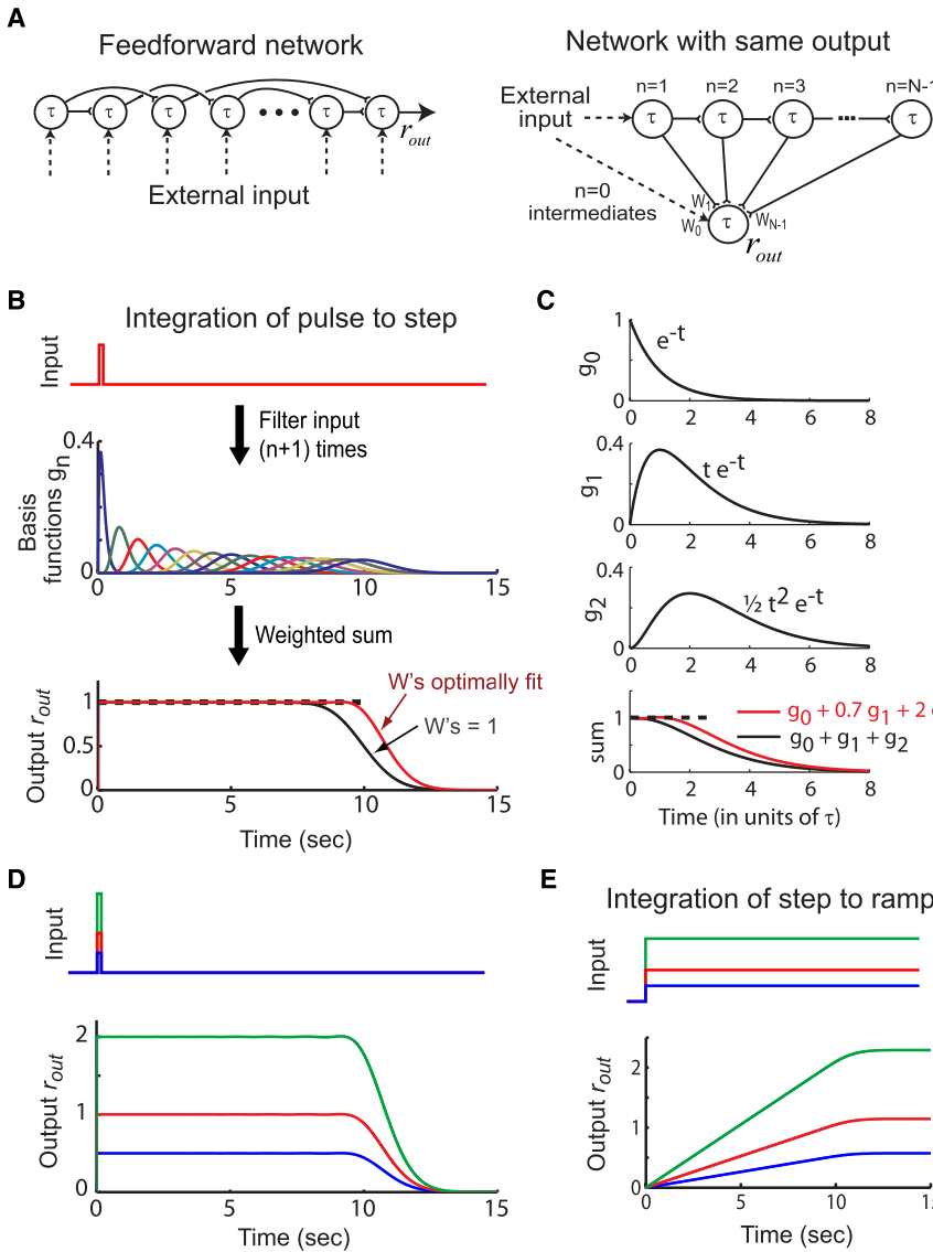
Figure 1. Integration by a Feedforward Network
