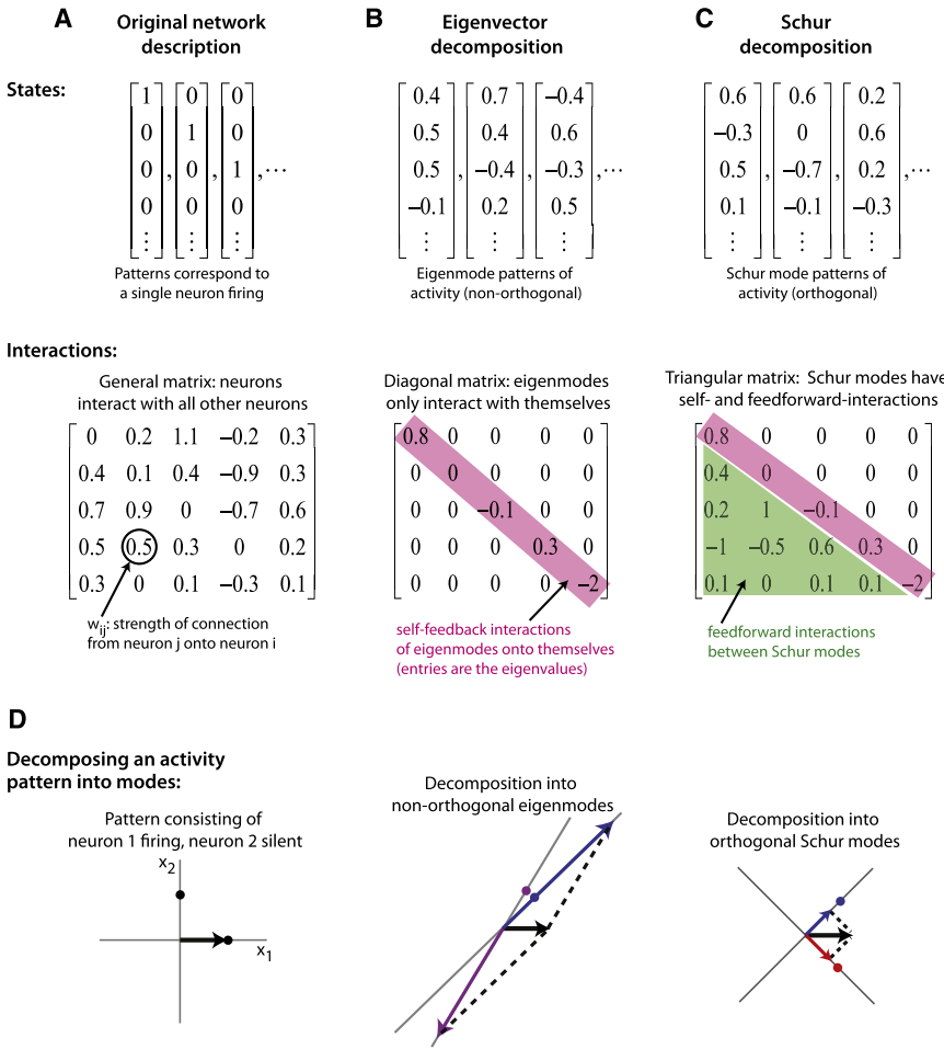
Figure 5. Comparison of the Eigenvector and Schur Decompositions
